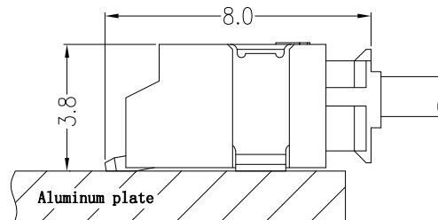
Assembly Layout
